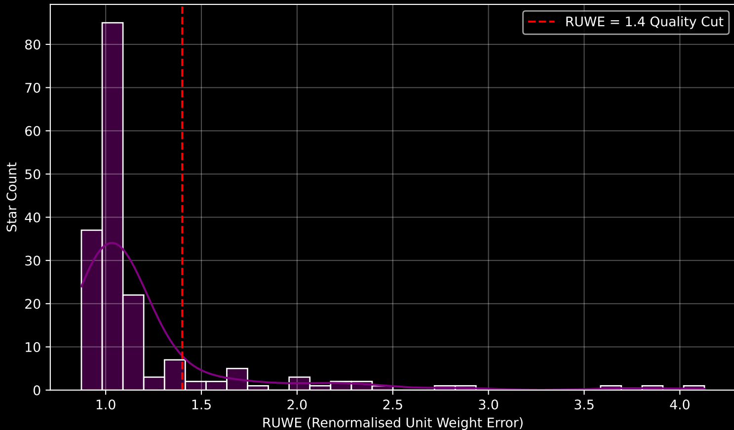
GALAH DR4 Field [301] RUWE Distribution (n= 178)
