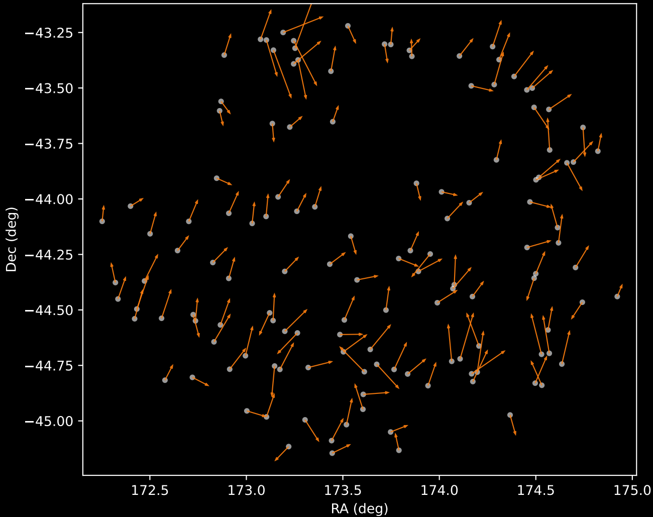
GALAH DR4 Cluster 2 Proper Motion Vectors (n=132)
