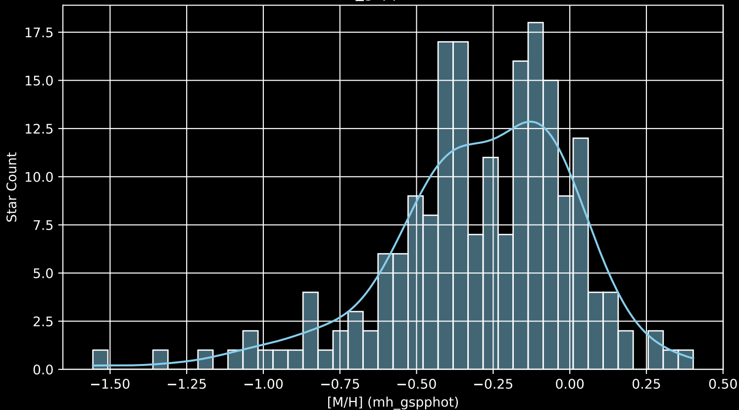
GALAH DR4 Field: [301] [M/H] (mh_gspphot) (n= 193)
