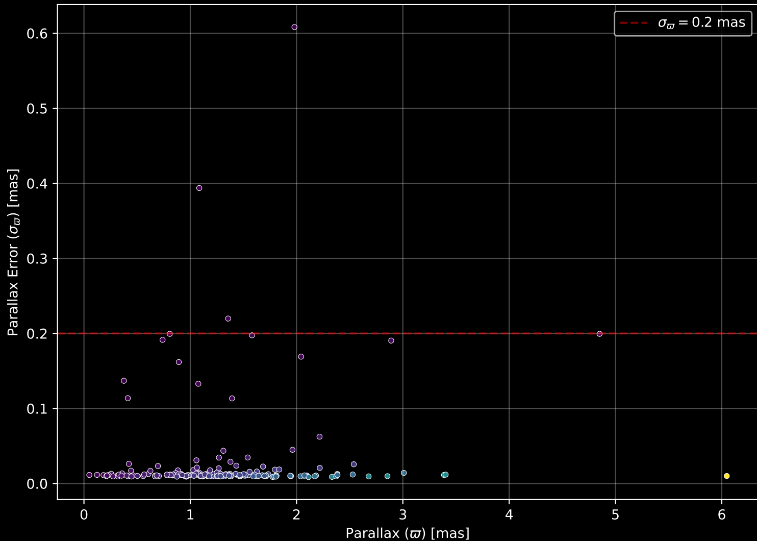
GALAH DR4 Field: [301] Parallax Quality (n= 193)
