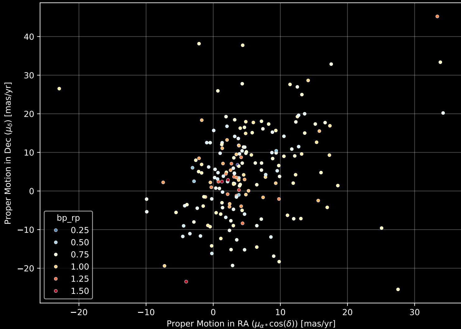
GALAH DR4 Field: [301] Proper Motion Diagram (n= 193)
